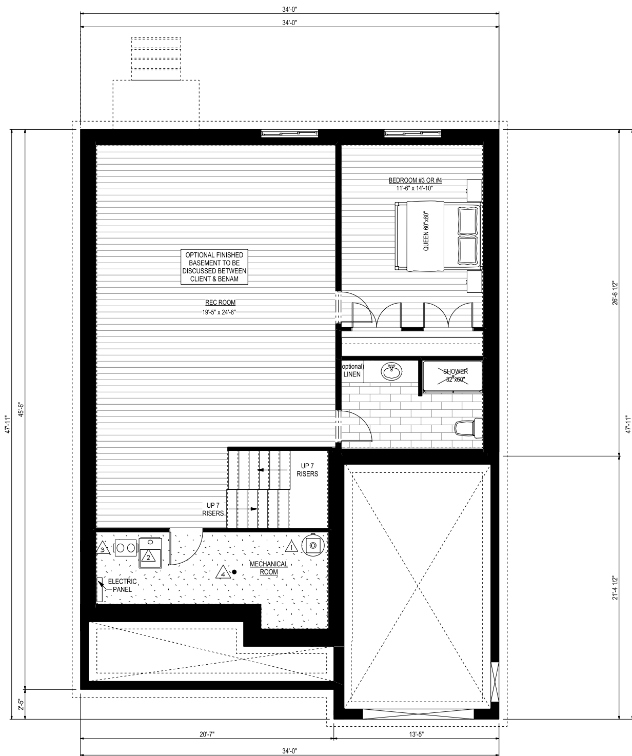
BASEMENT PLAN
