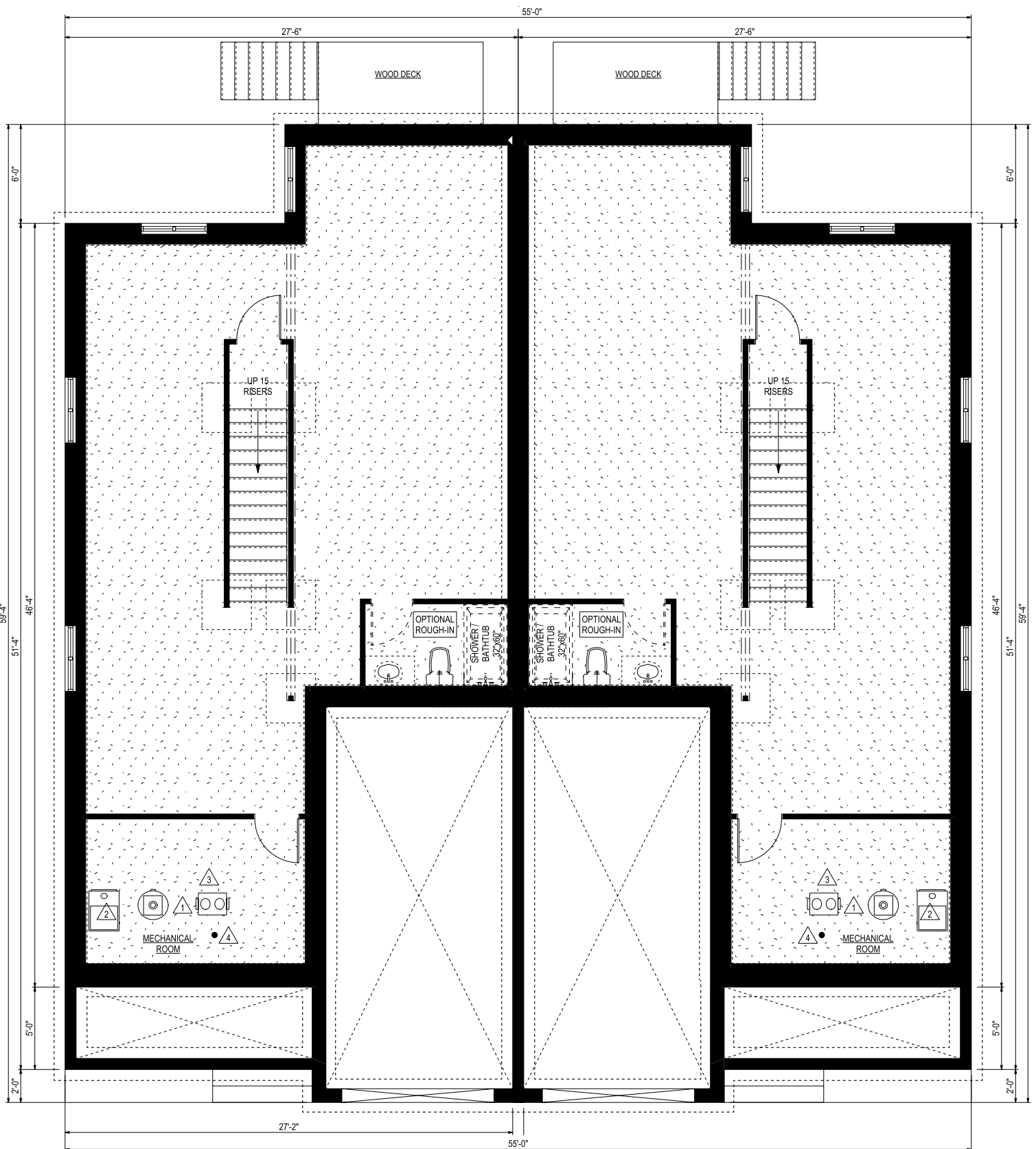
BASEMENT PLAN
