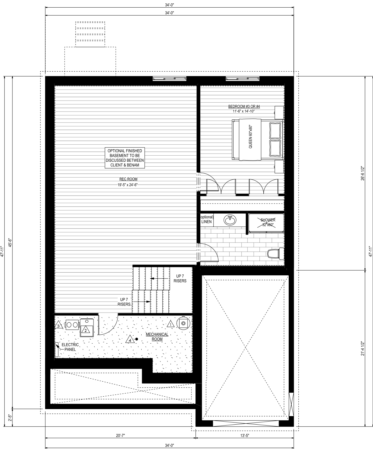
BASEMENT PLAN
