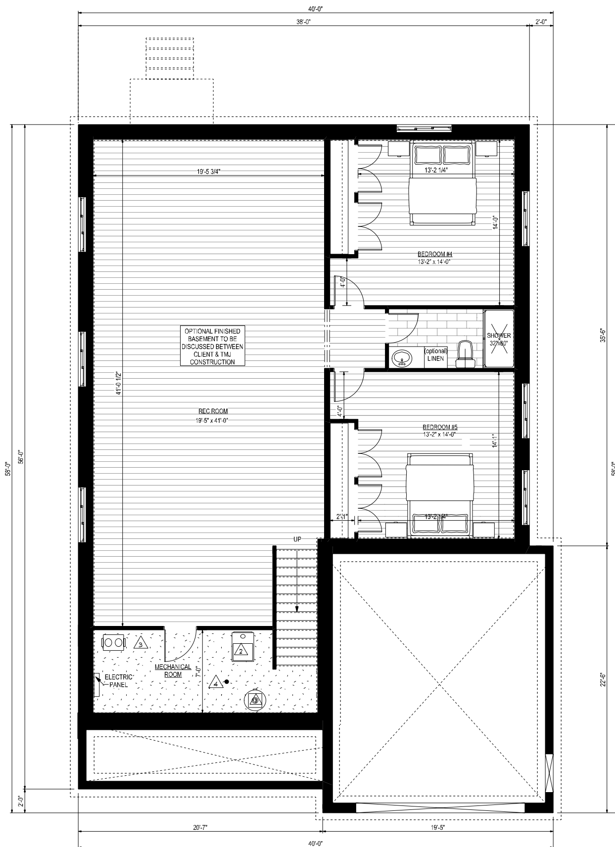
BASEMENT PLAN
