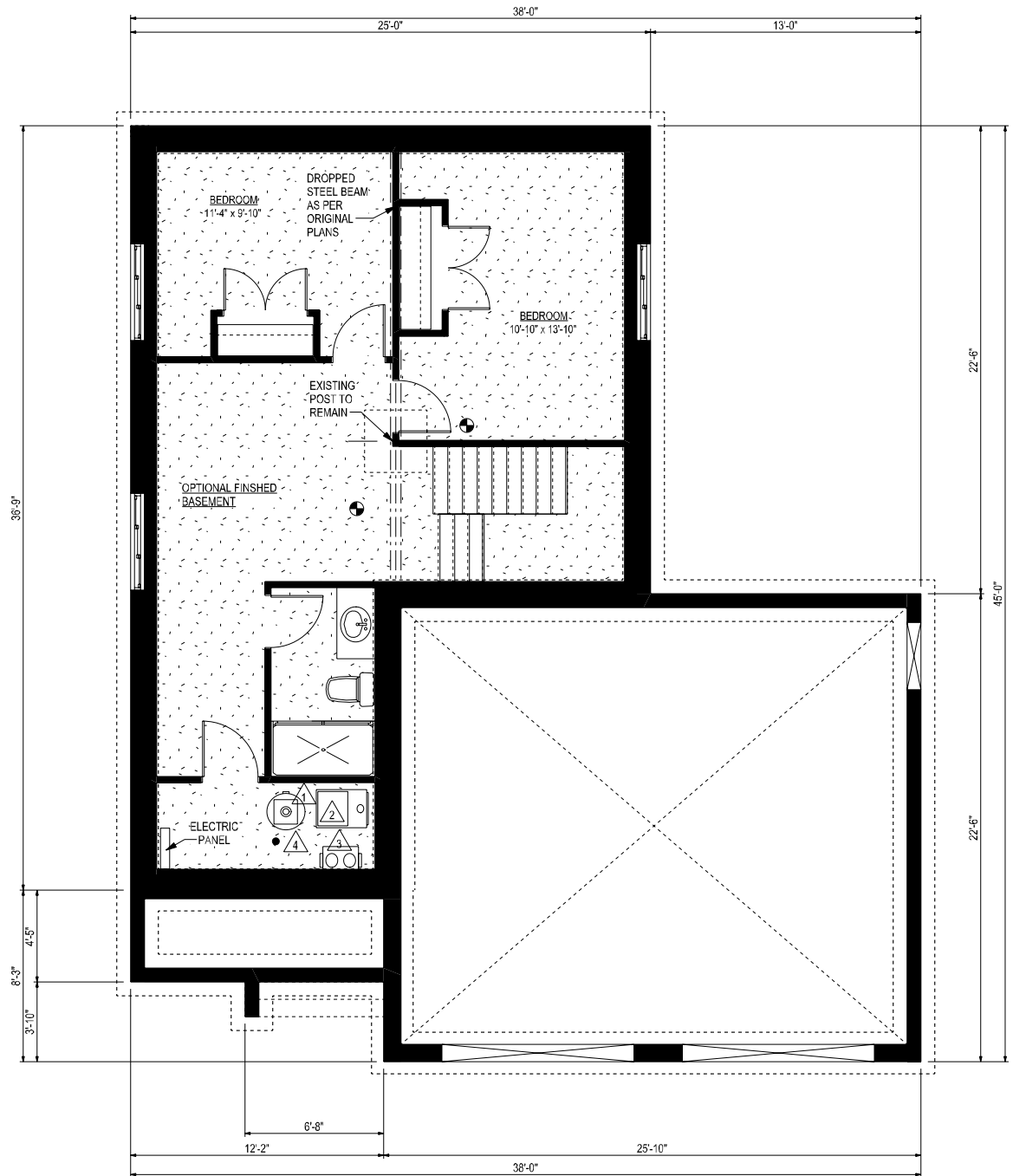
BASEMENT PLAN
