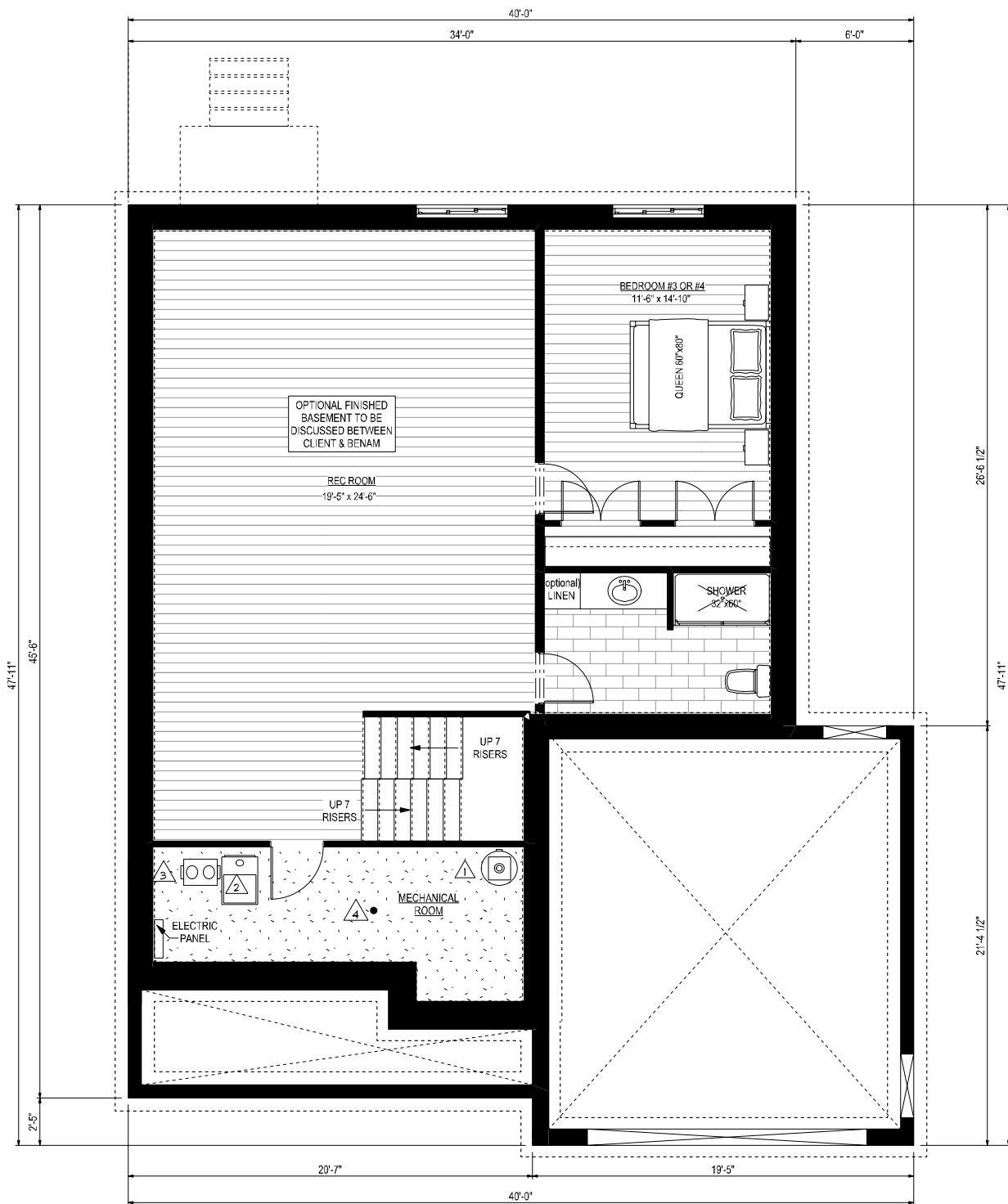
BASEMENT PLAN
