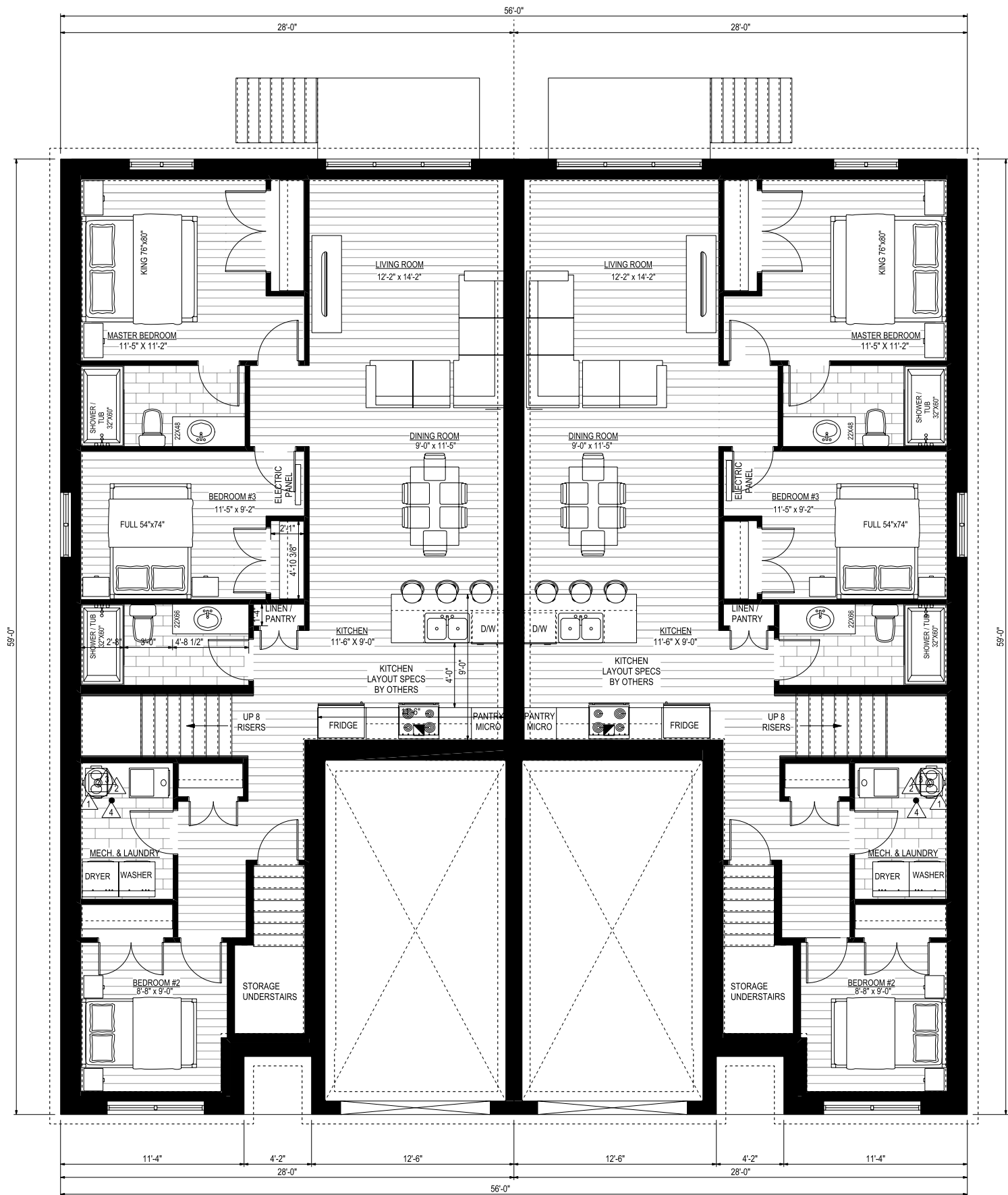
BASEMENT PLAN
