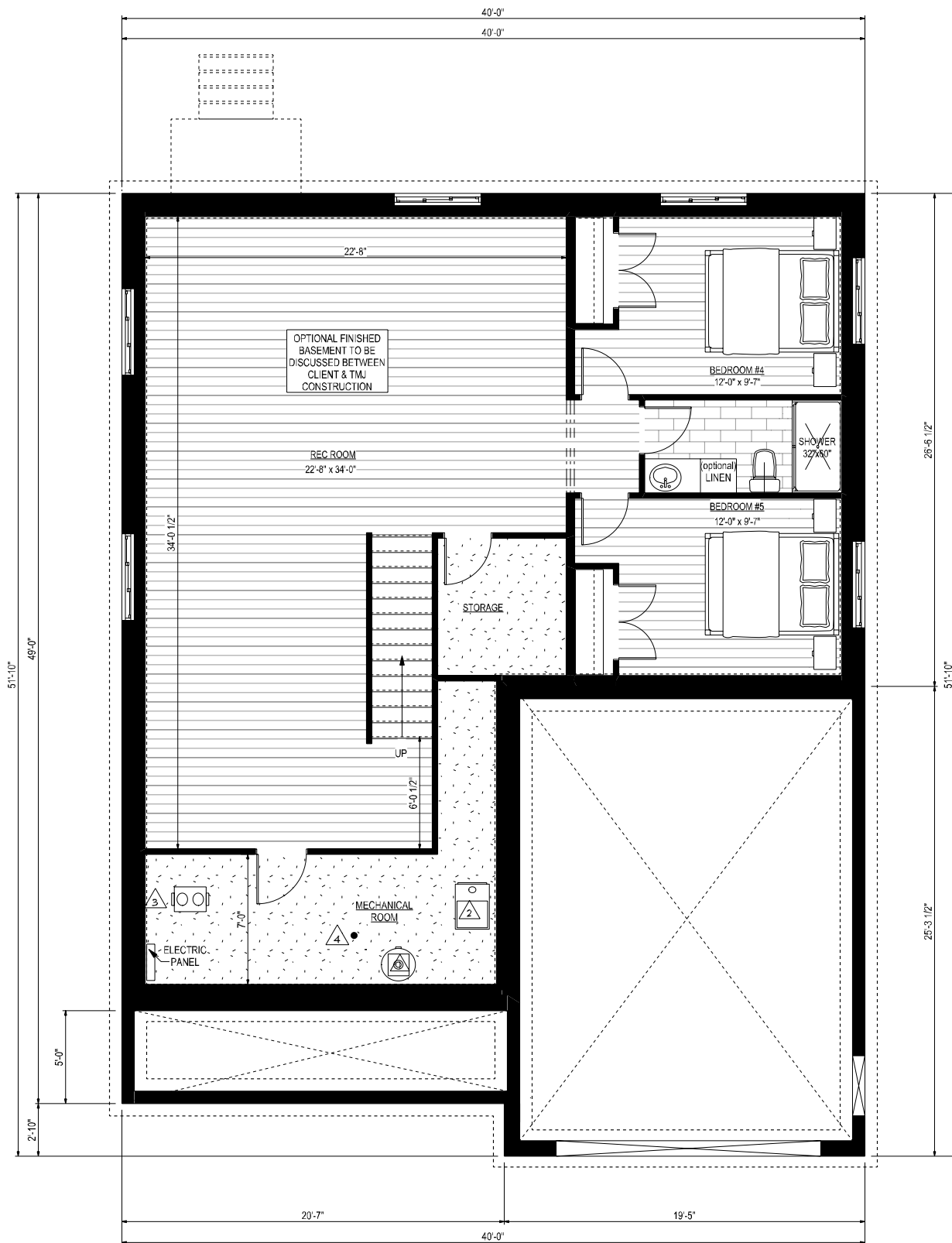
BASEMENT PLAN
